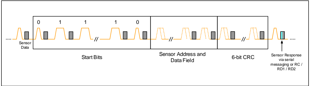
Figure 7: ECU to sensor communication with Pulse Width method
