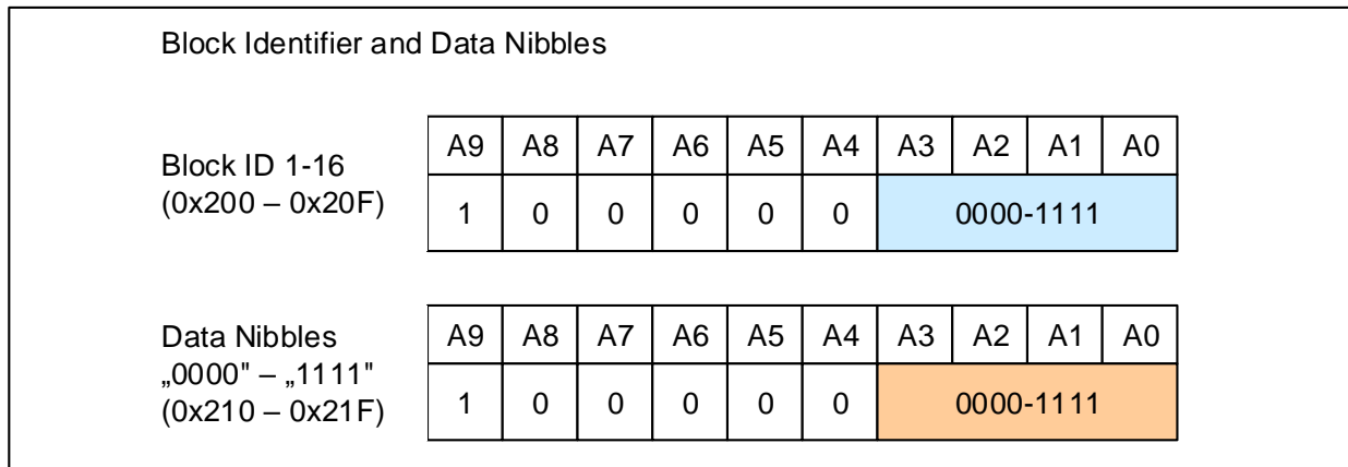
Figure 35: Block ID and data nibbles
