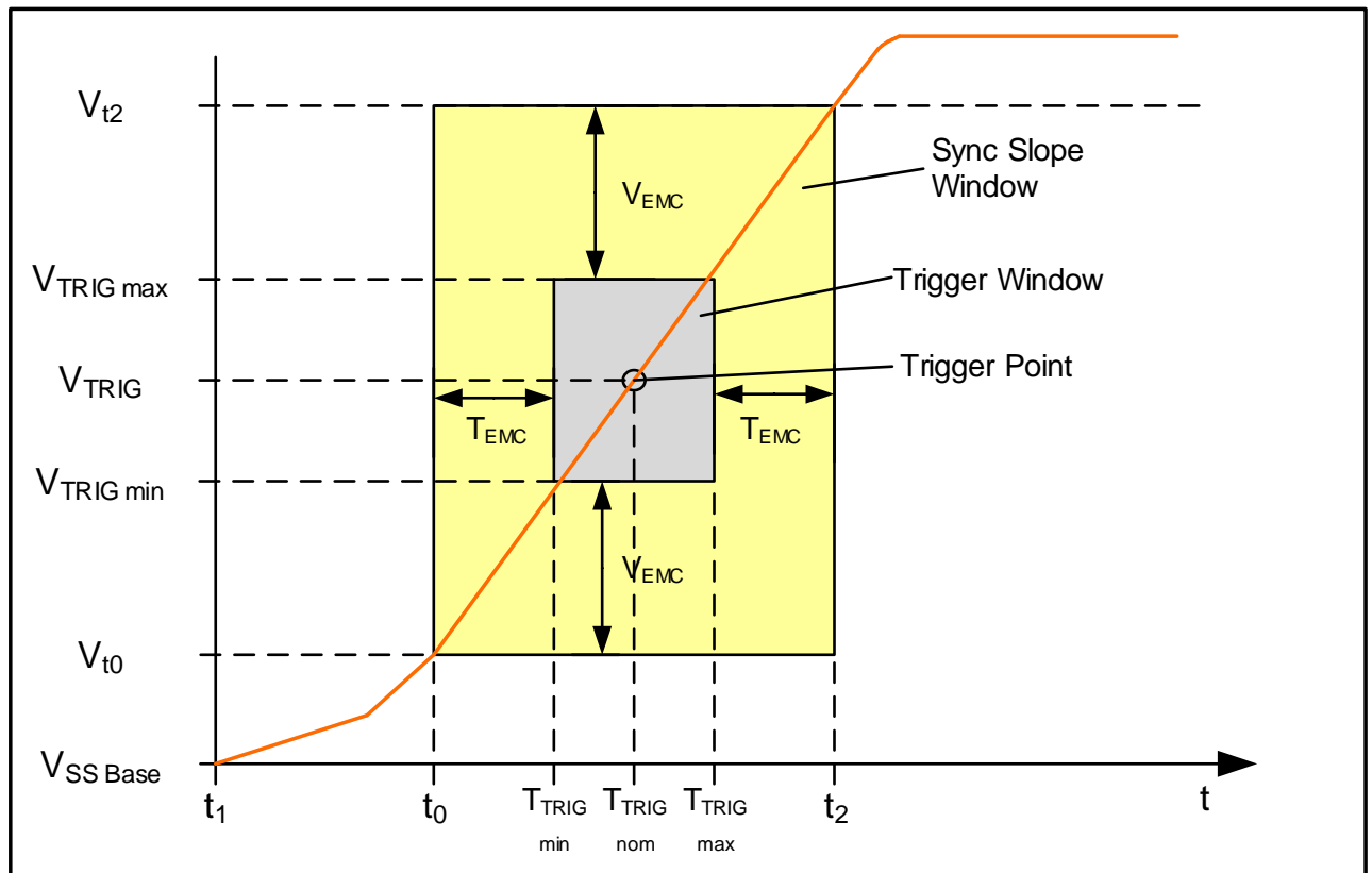
Figure 28: Synchronization signal detection in the sensor
