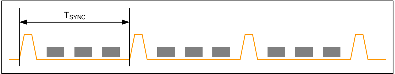
Figure 40: Fixed time triggered synchronous operation
