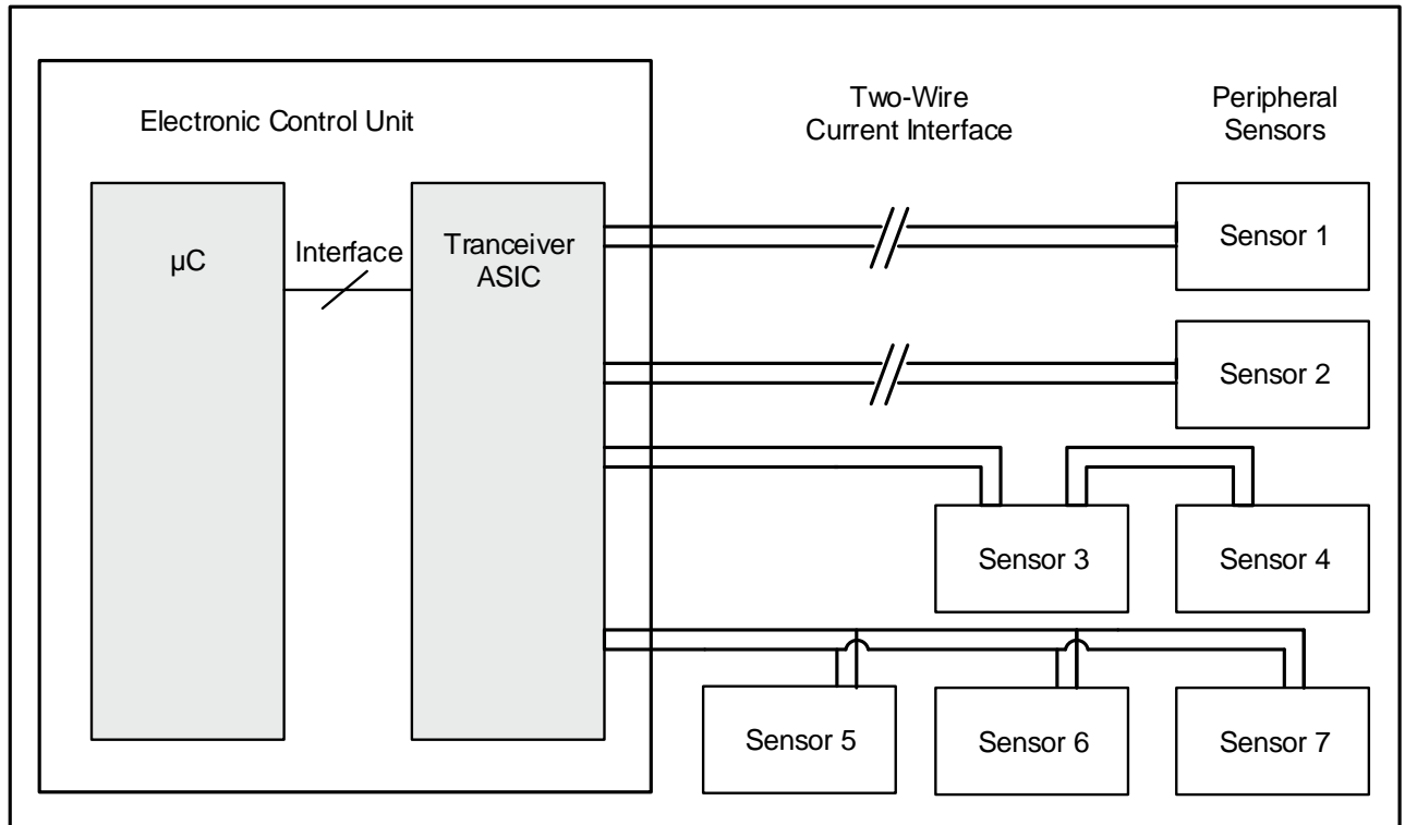
Figure 37: Connection of peripheral sensors to an ECU (Example)
