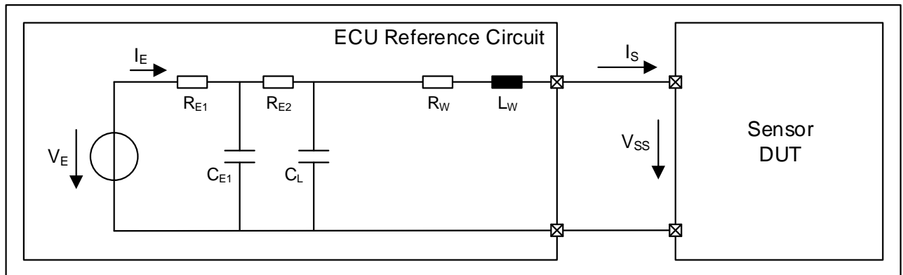
Figure 24: Reference circuit for sensor testing
