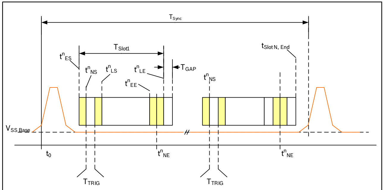
Figure 29: Timing of synchronous operation
