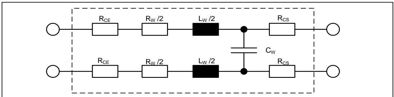
Figure 13: Supply line model for PSI5
