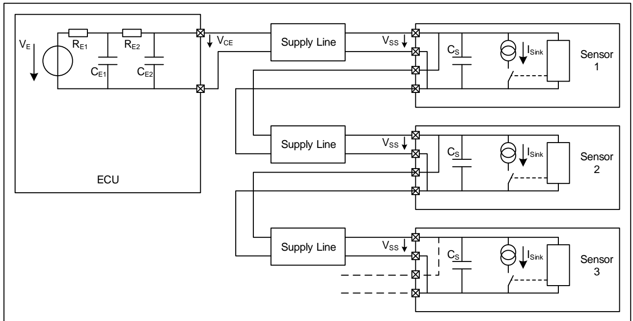
Figure 16: Example for a pass-through configuration (simplified schematic)
