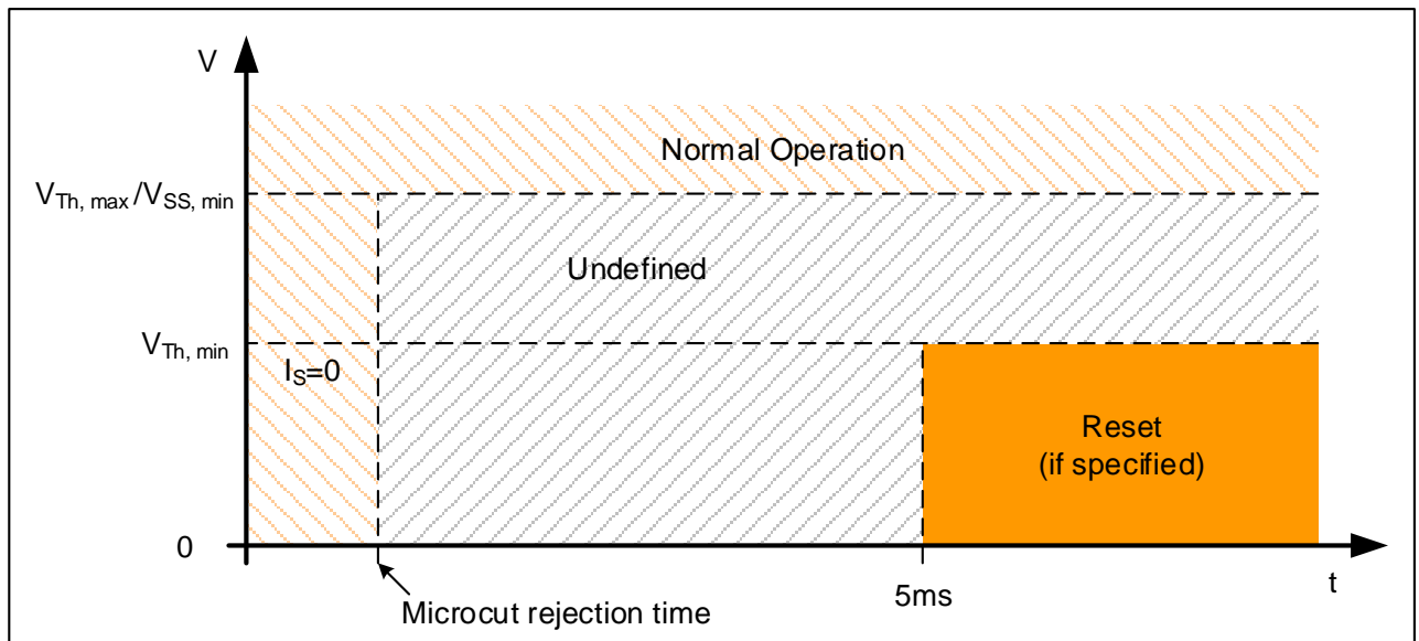
Figure 32: Undervoltage reset behavior
