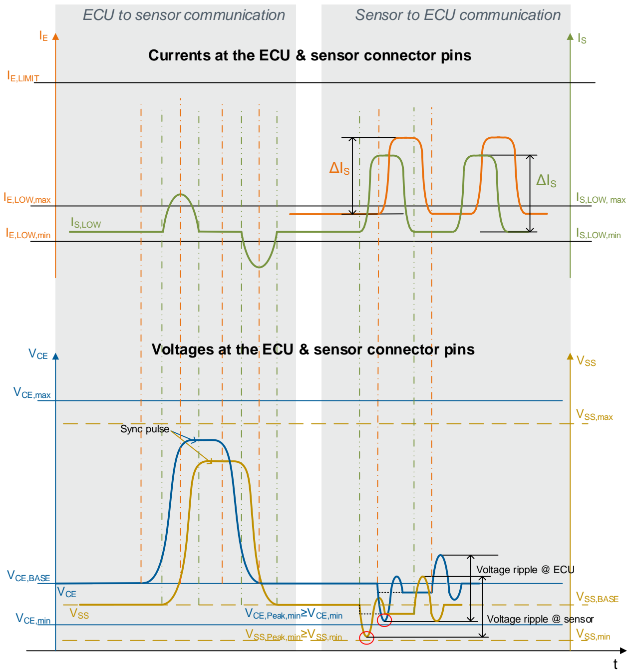
Figure 22: System current and voltage definitions
