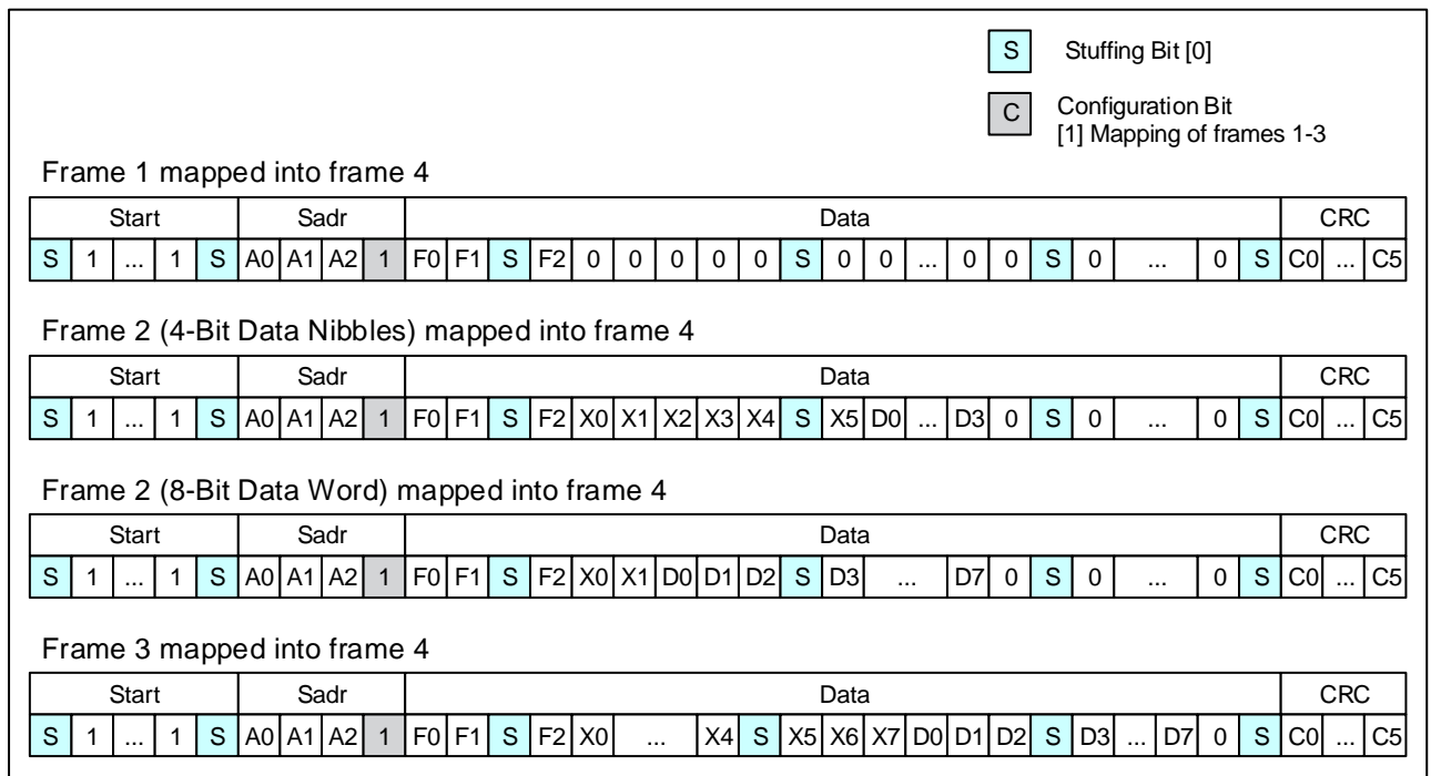
Figure 9: Mapping of frames 1-3 into frame 4
