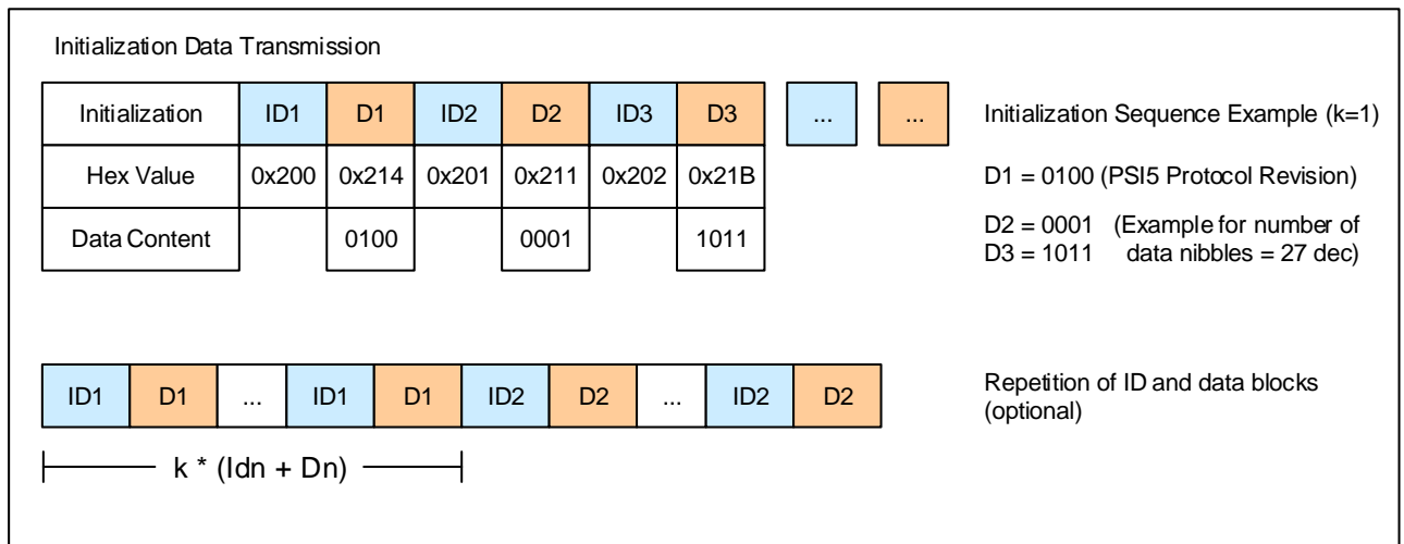
Figure 36: Startup sequence
