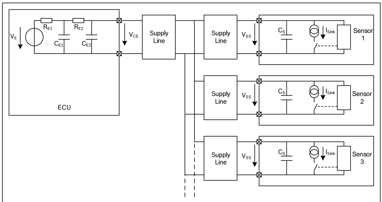
Figure 17: Example for a splice configuration (simplified schematic)
