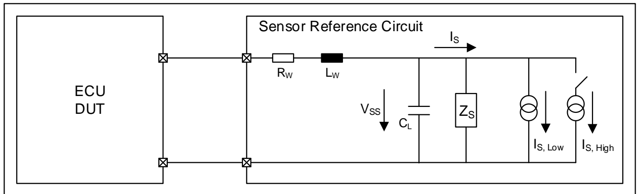
Figure 25: Reference circuit for ECU testing
