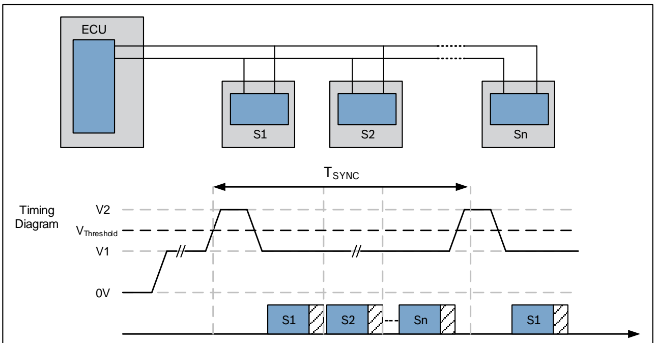
Figure 42: Basic PSI5 bus topology
