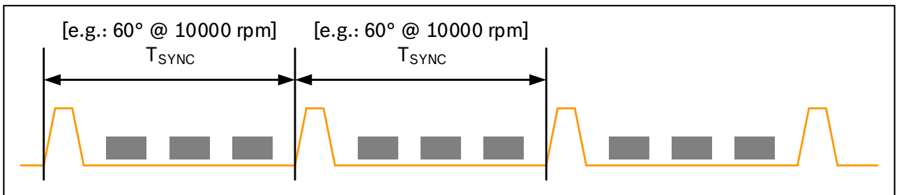
Figure 41: Variable time triggered synchronous operation
