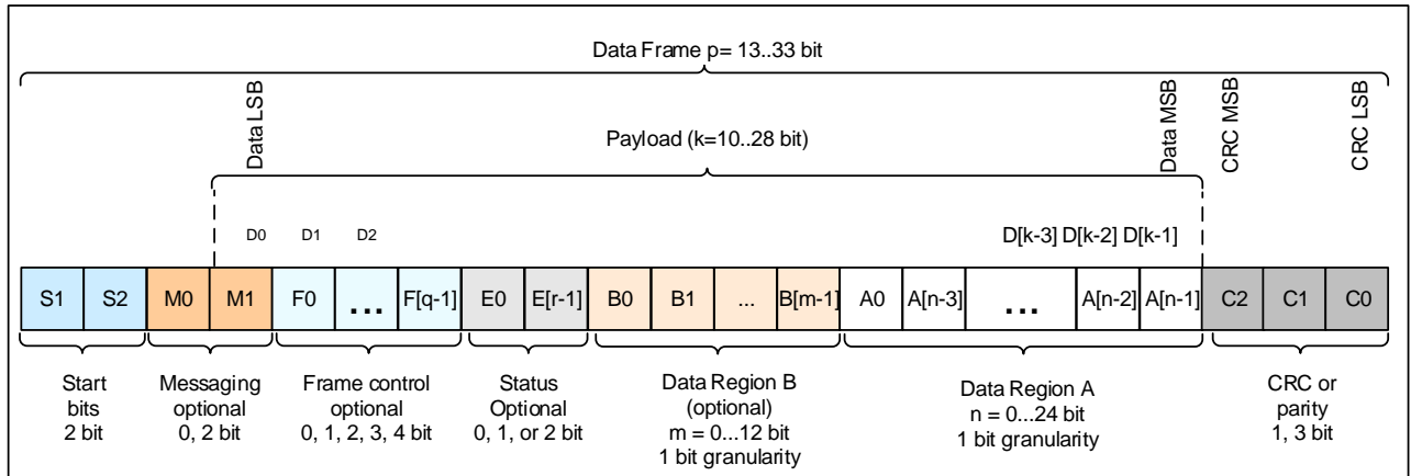
Figure 2: Different parts of the PSI5 data frame
