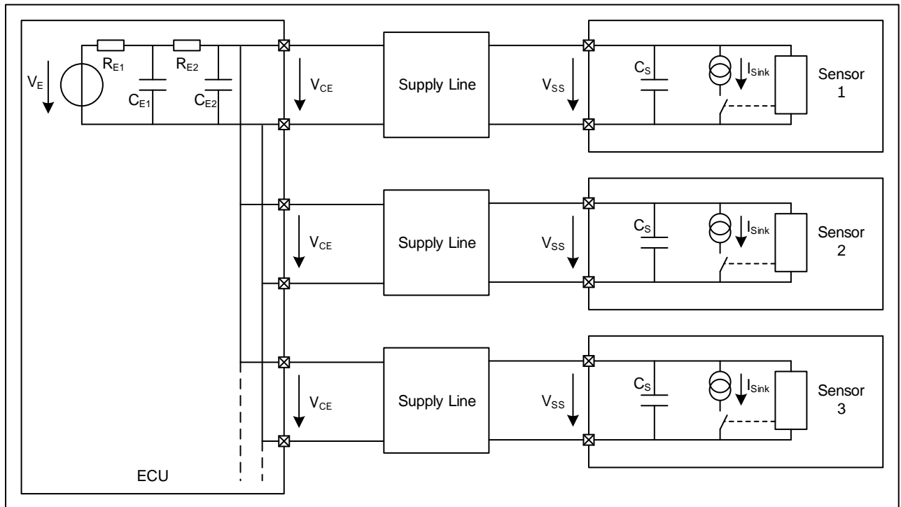
Figure 15: Synchronous parallel bus mode (simplified schematic)
