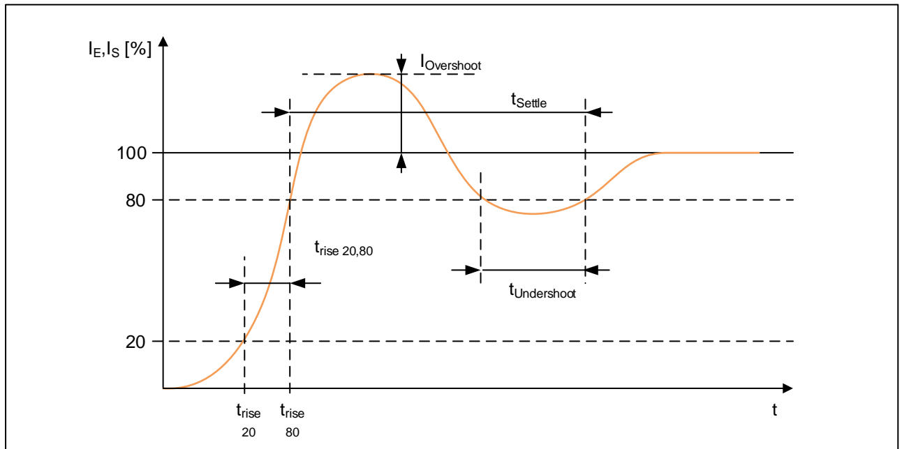
Figure 26: Dynamic behavior of supply / communication current
