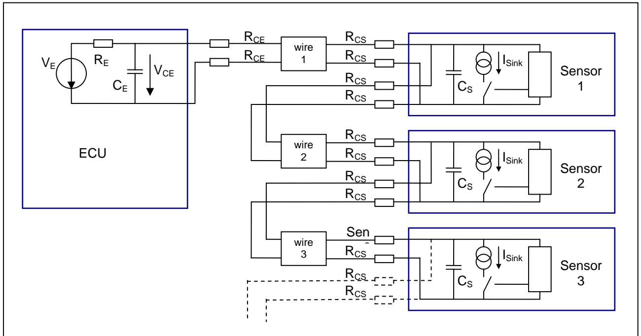
Figure 8 Example for a pass-through configuration (simplified schematic)
