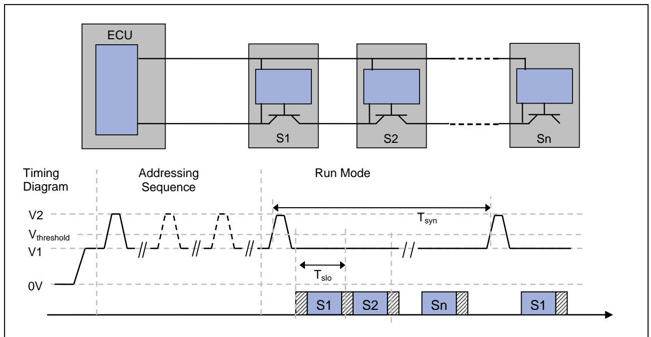
Figure 6 Daisy Chain Bus Topology
