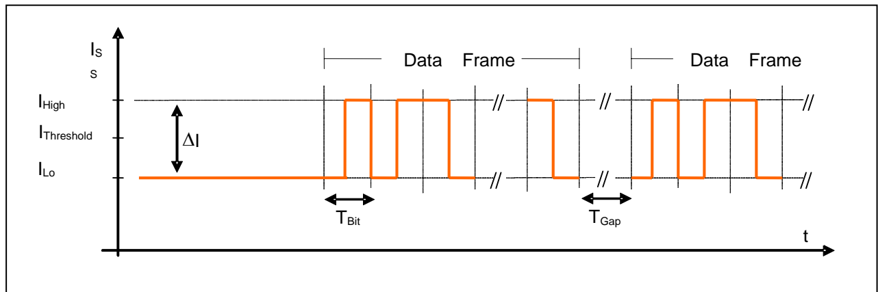
Figure 22 Data frame timing
