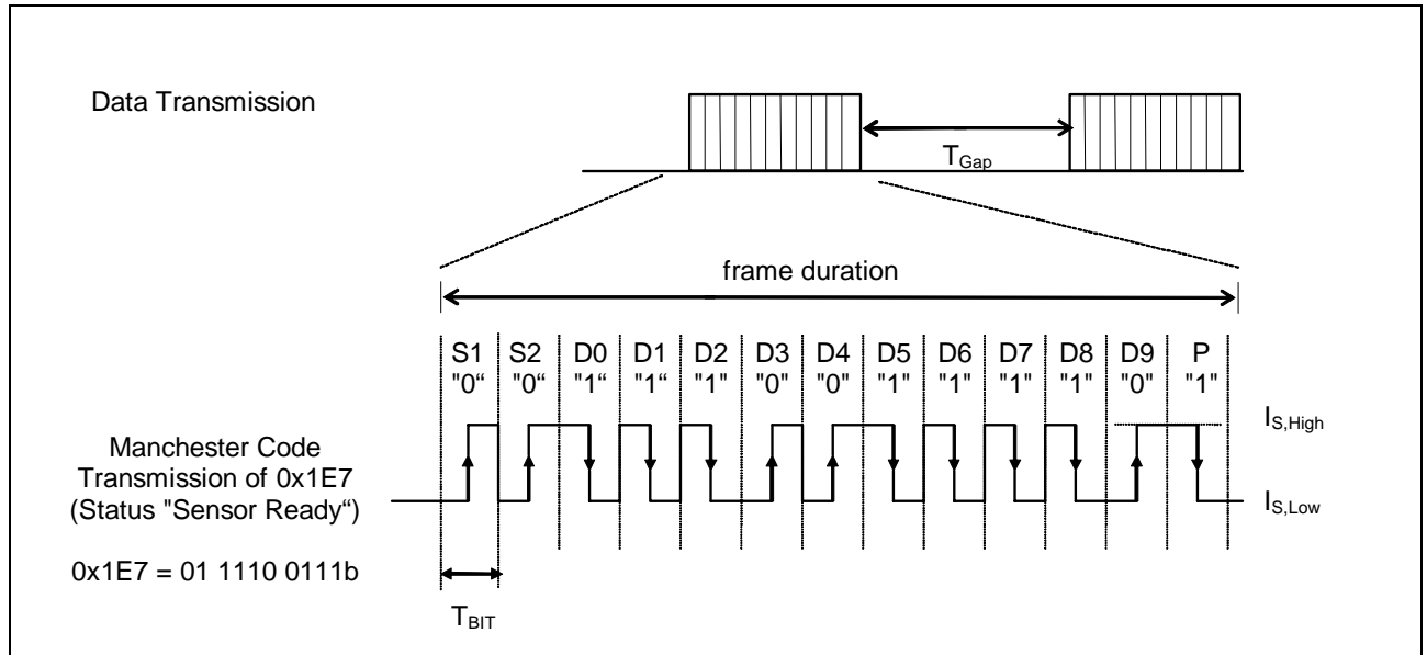
Figure 12 Example of a data frame with 10 data bits (D0-D9), 2 start bits (S1,S2) and one parity bit (P).
