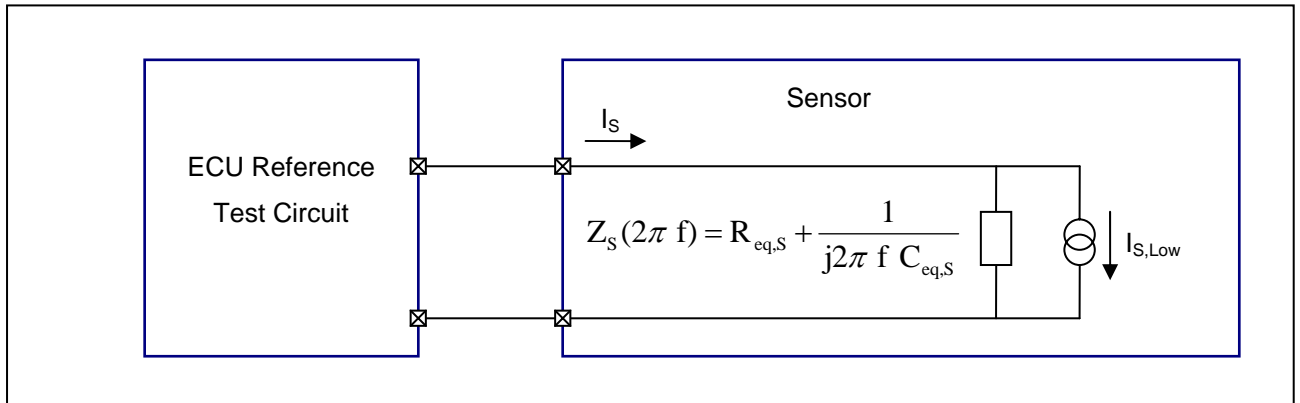
Figure 28 Reference circuit for sensor damping behaviour
