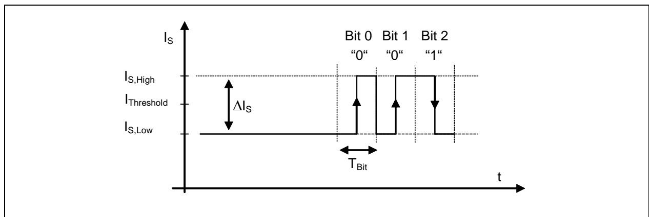
Figure 11 Bit encoding using supply current modulation
