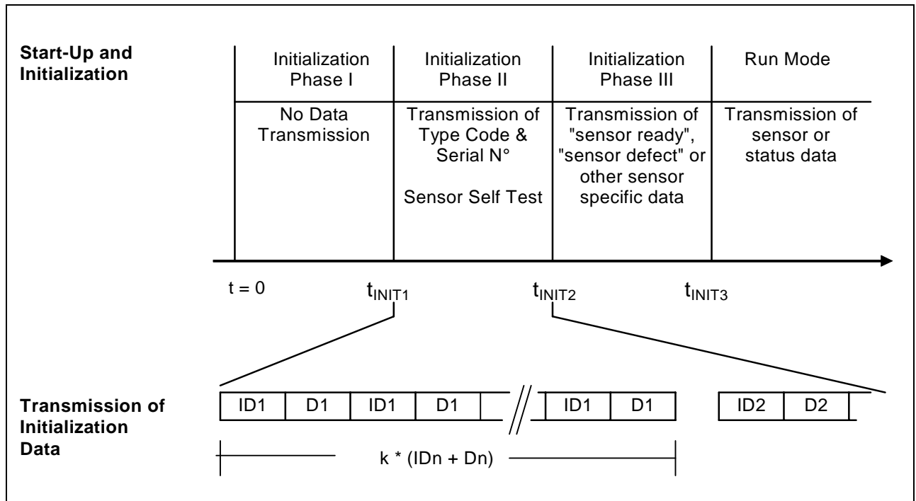
Figure 15 Initialization of the sensor
