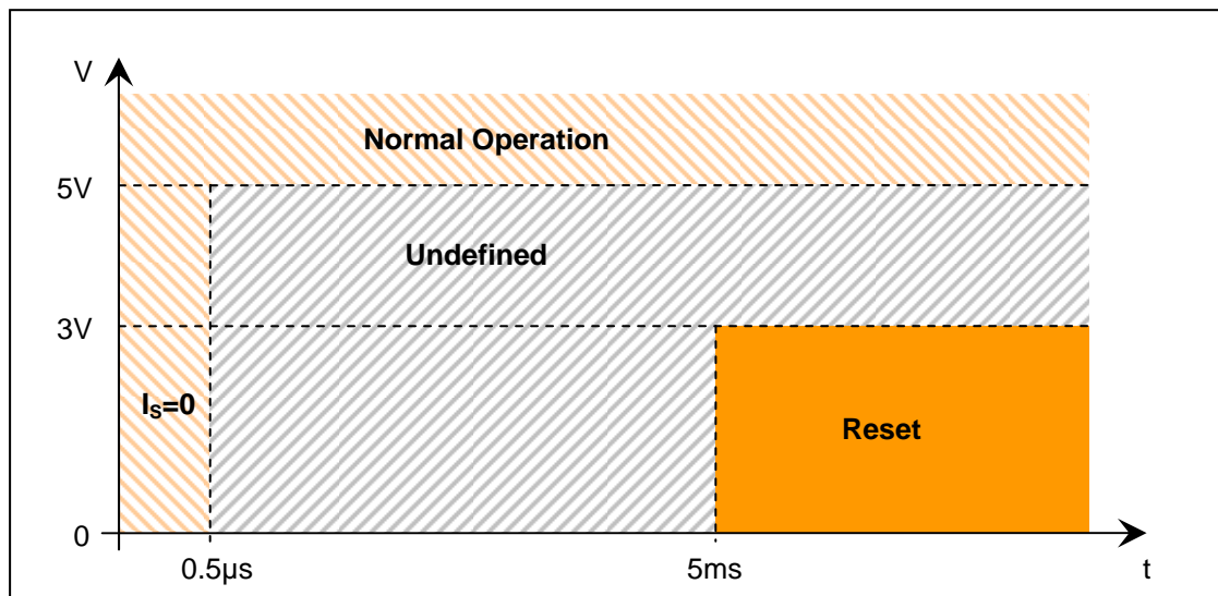
Figure 21 Undervoltage reset behaviour
