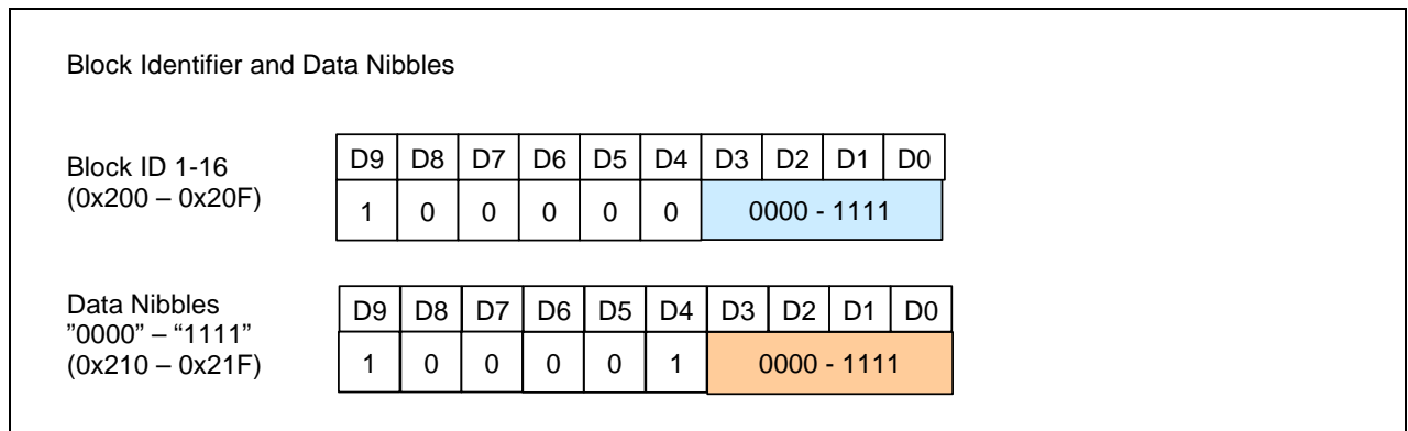
Figure 16 Block ID and Data Nibbles
