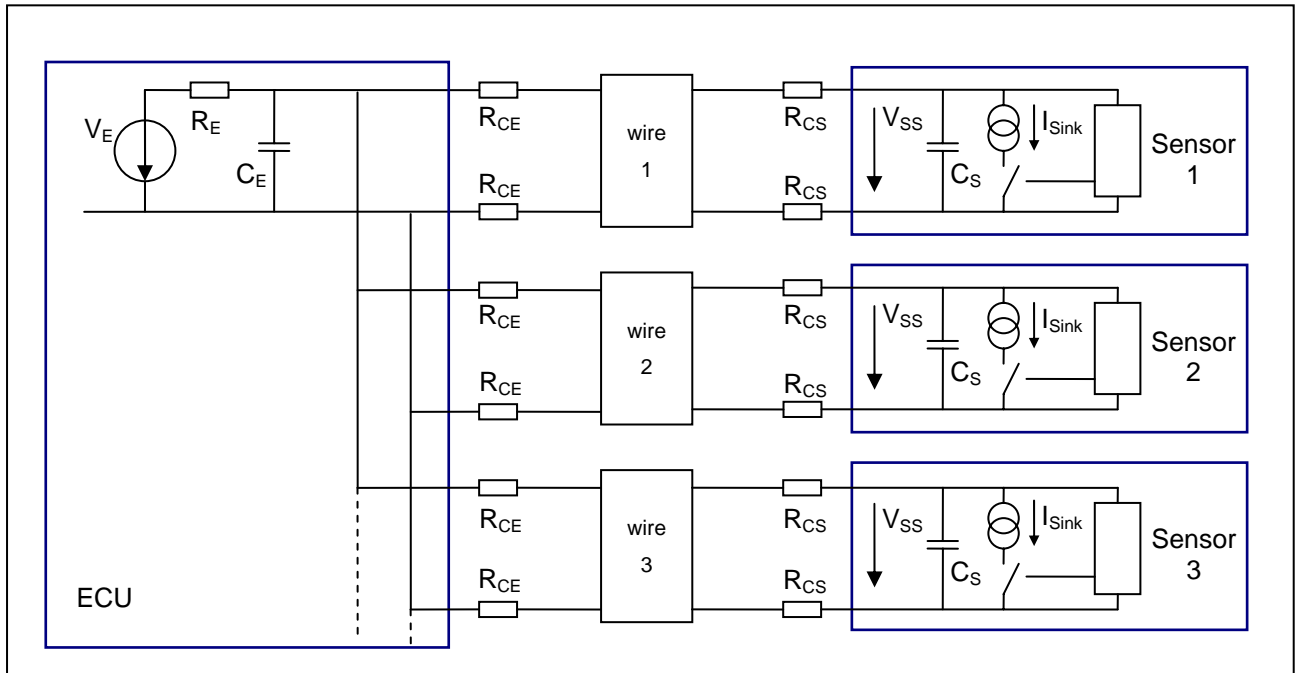
Figure 7 Synchronous Parallel Bus Mode (simplified schematic)
