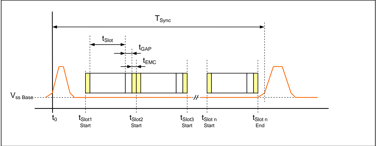
Figure 25 Timing of synchronous operation
