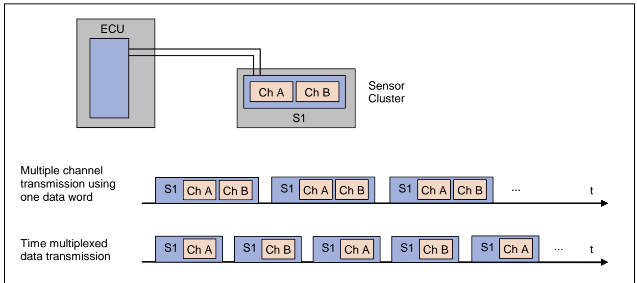
Figure 10 Sensor cluster
