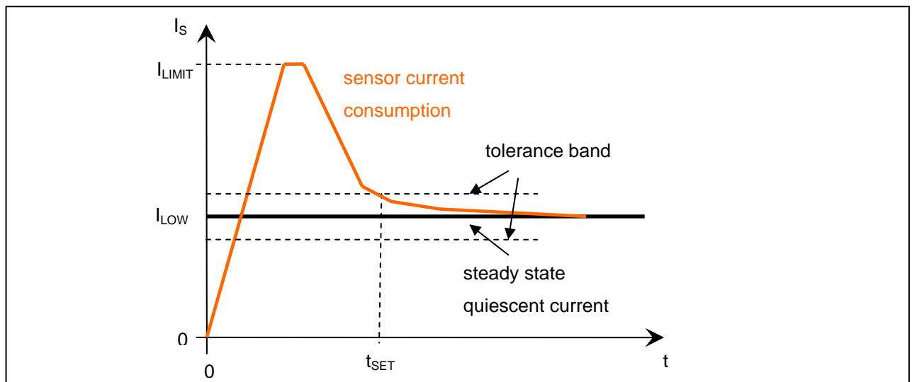
Figure 20 Current consumption during startup
