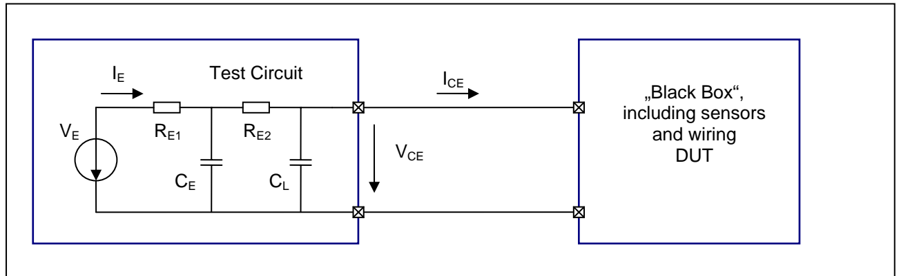
Figure 29 Reference test bench for bus testing
