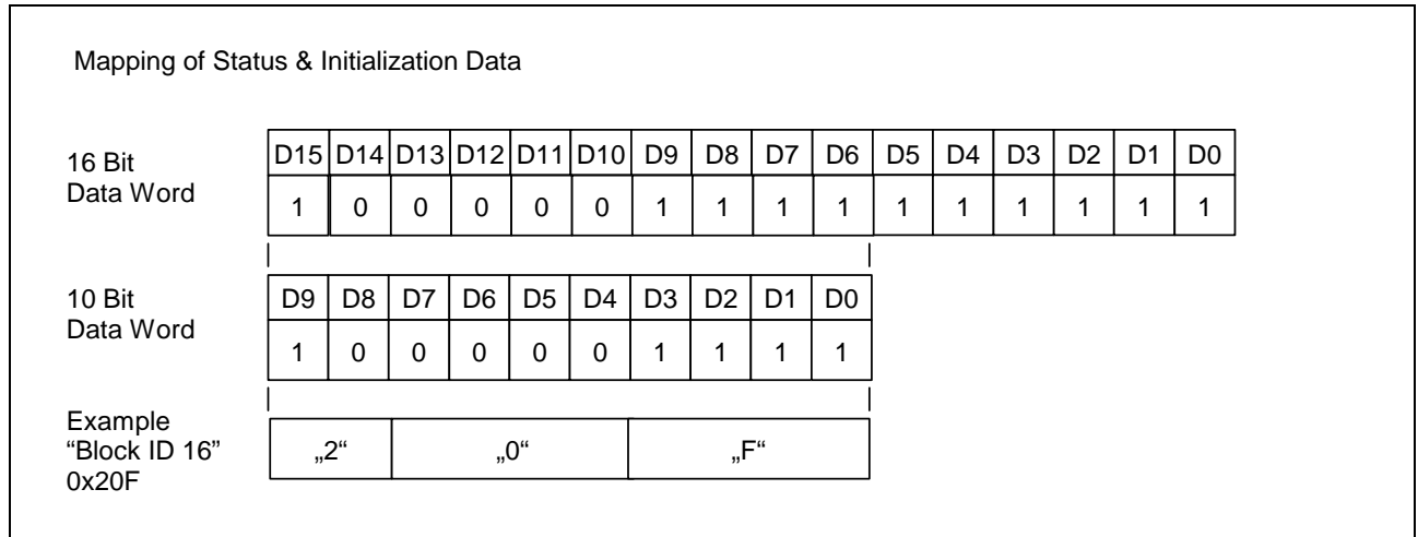
Figure 14 Mapping of status and initialization data into a data word
