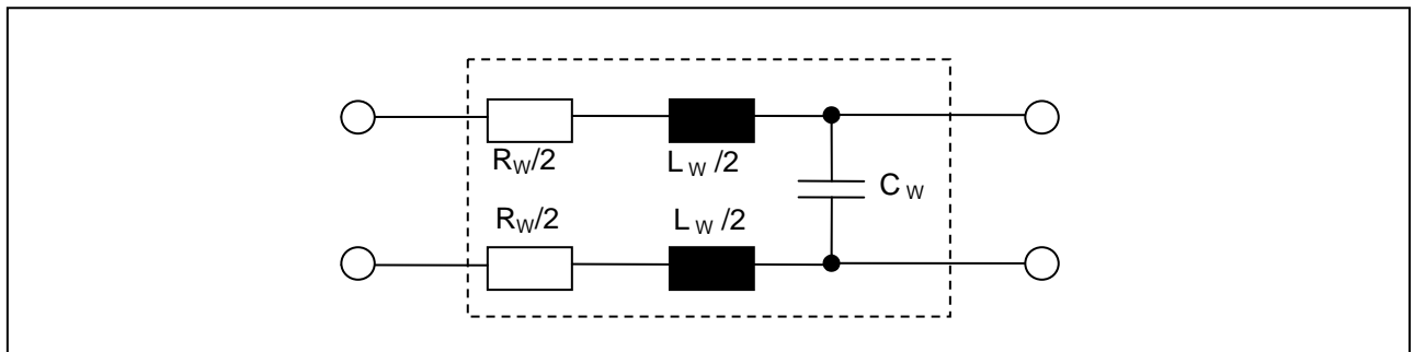
Figure 26 Supply line model for PSI5
