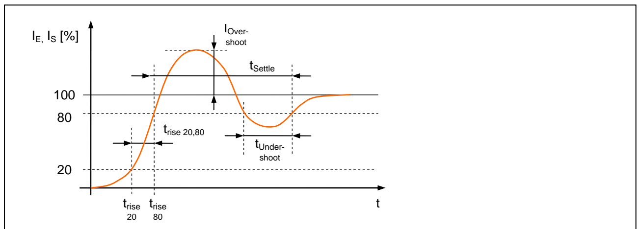
Figure 30 Test parameter sending current
