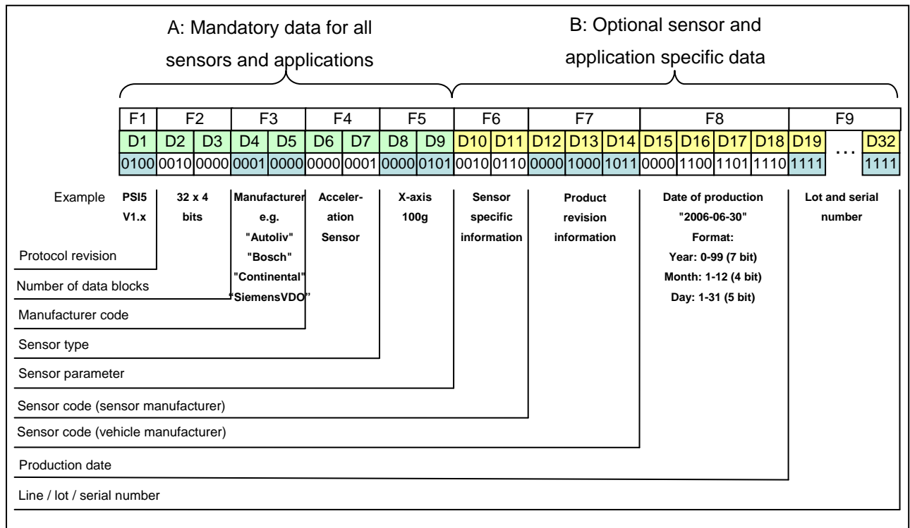
Figure 18 Initialization phase 2: Recommended Data Content
