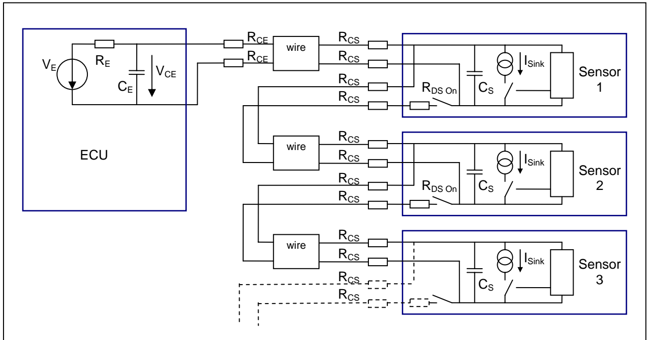
Figure 9 Synchronous Daisy Chain Bus (simplified schematic)
