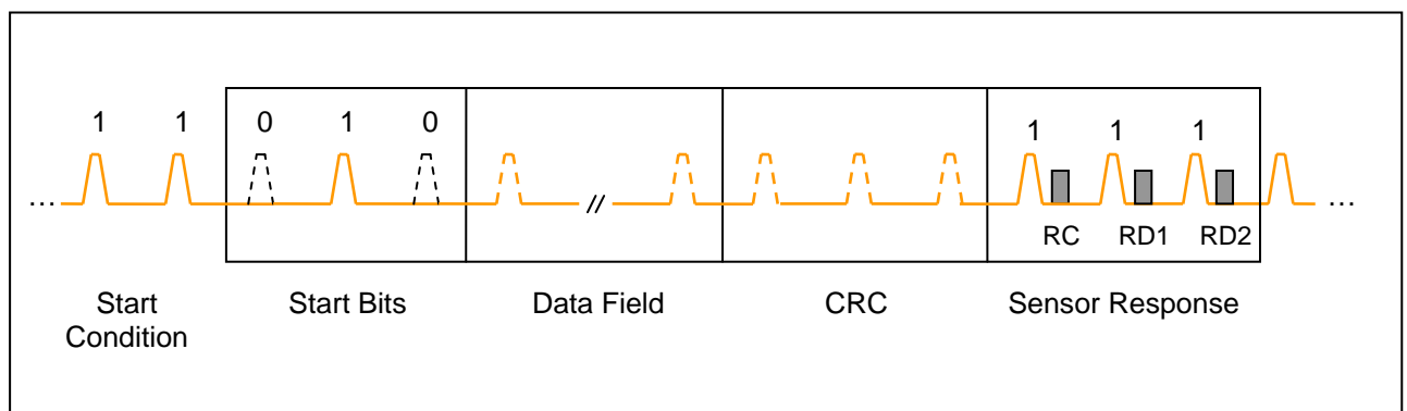
Figure 19 Data frame ECU to sensor communication
