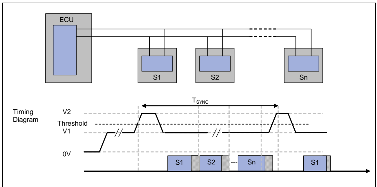
Figure 5 Basic PSI5 bus topology
