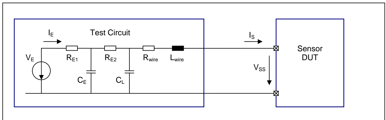
Figure 27 Reference test bench for sensor testing
