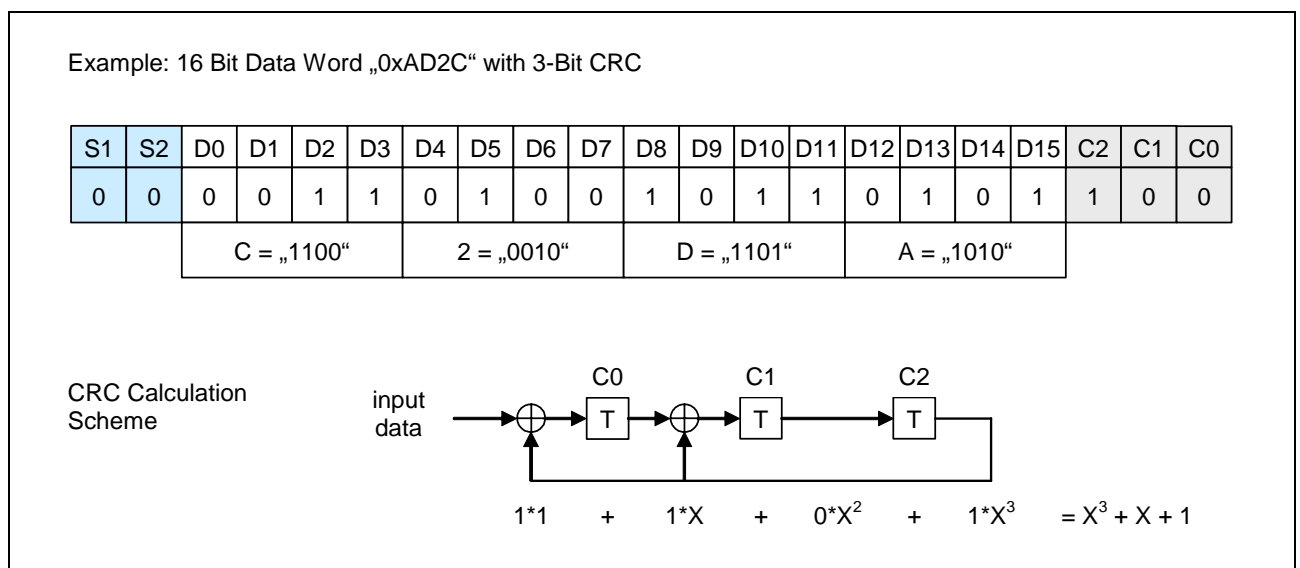
Figure 13 16 Bit Data word example with 3-Bit CRC
